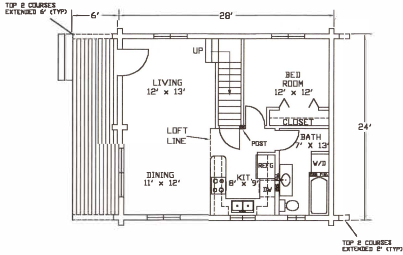
MAIN FLOOR PLAN = 672 SQ. FT.
