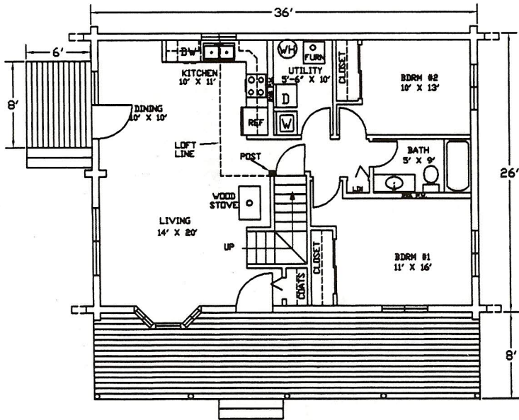
MAIN FLOOR 936 SQ. FT. SCALE: 1/4" = 1'-0"
