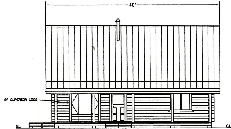
FRONT VIEW SCALE: 1/4" = 1'-0"
