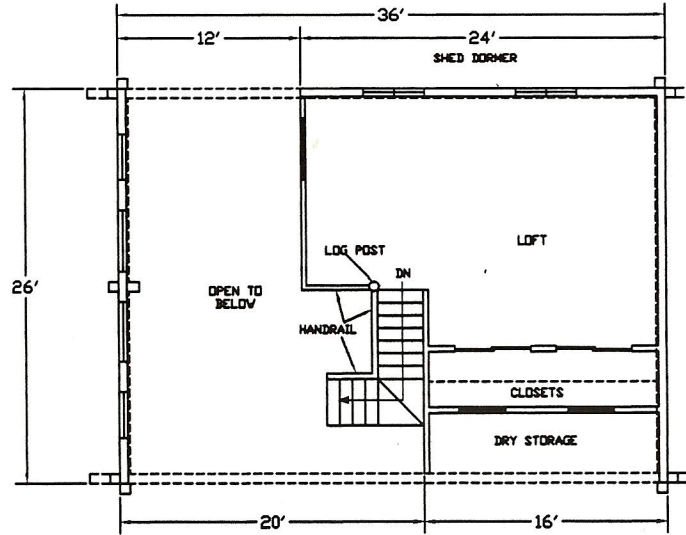
LOFT 440 SQ. FT. SCALE: 1/4" = 1'-0"
