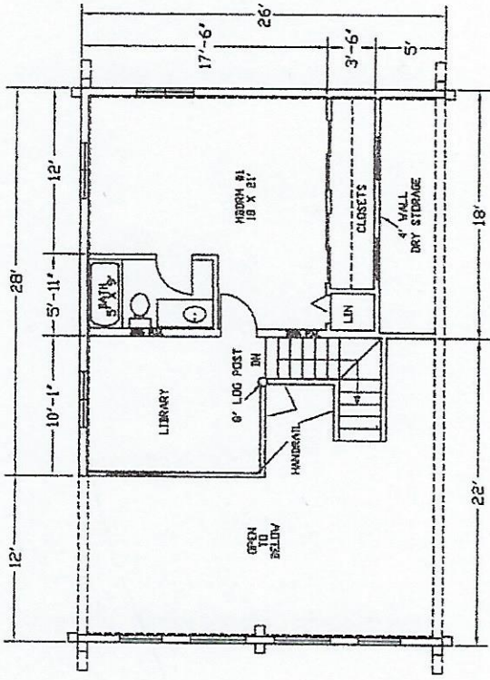
LOFT FLOOR PLAN 520 SQ. FT. SCALE 1/4" = 1'-0"
