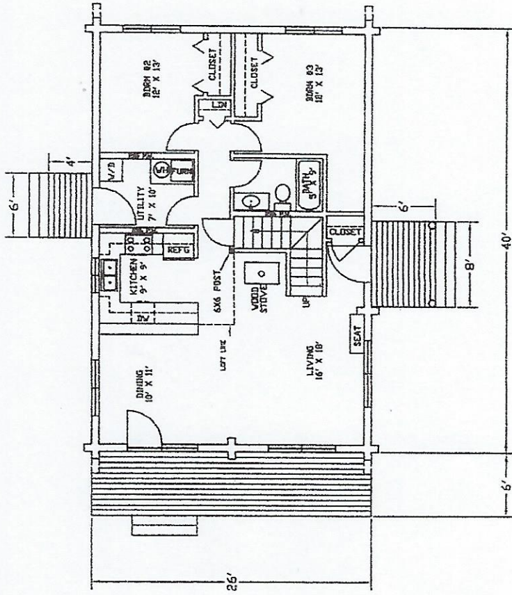
FIRST FLOOR PLAN 1,040 SQ. FT. SCALE 1/4" = 1'-0"
